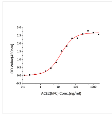
Immobilized SARS-CoV-2 Spike RBD(L452R,T478K)(Avi) at 2 \mu g/mL (100 \mu L/well) can bind Human ACE2 (Catalog: RP01275) with a linear range of 0.1-14.28 ng/mL.
