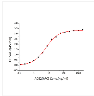
Immobilized SARS-CoV-2 Spike RBD (Lambda/C.37)(Avi) at 2 \mu g/mL (100 \mu L/well) can bind Human ACE2 (Catalog: RP01275) with a linear range of 0.1-6.43 ng/mL.
