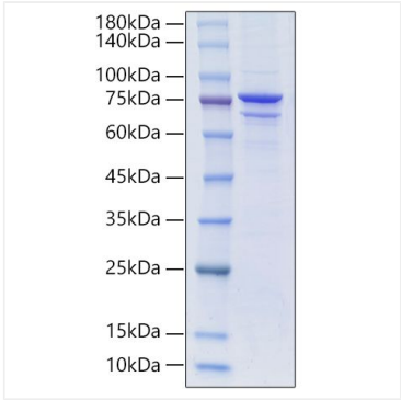
Recombinant African swine fever virus P72/B646L&B602L Protein was determined by SDS-PAGE under reducing conditions with Coomassie Blue.
