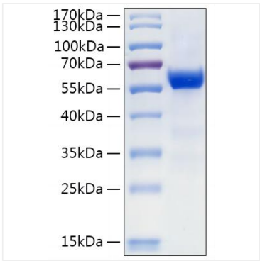
Recombinant Rat IL-6RA/CD126 Protein was determined by SDS-PAGE under reducing conditions with Coomassie Blue.
