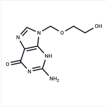
Chemical structure of Acyclovir(阿昔洛韦)(阿昔洛韦), CAS No.59277-89-3
