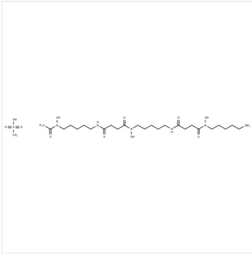
Chemical structure of Deferoxamine Mesylate(□□□□□)(□□□□),CAS No.138-14-7
